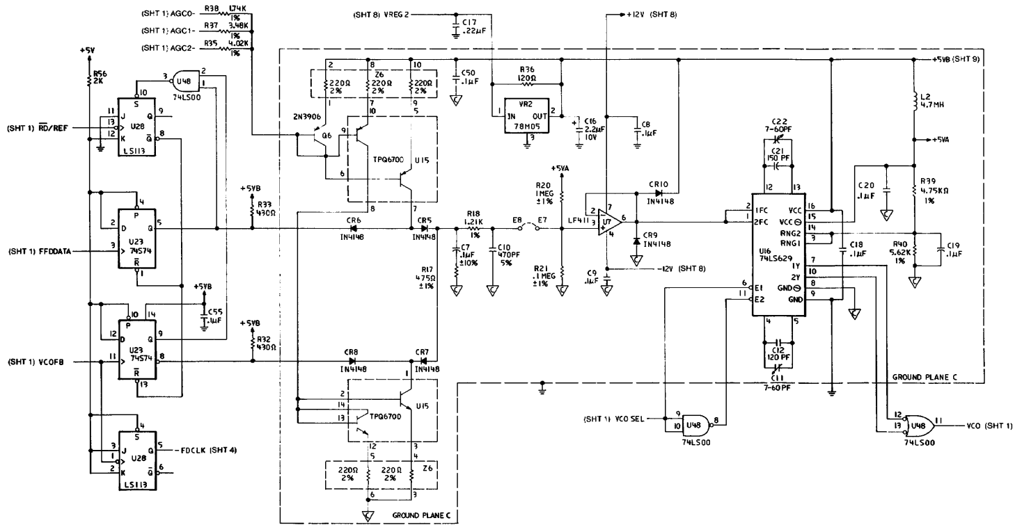
Fixed Disk and Diskette Drive Adapter - Level 1 (Sheet 9 of 9)
