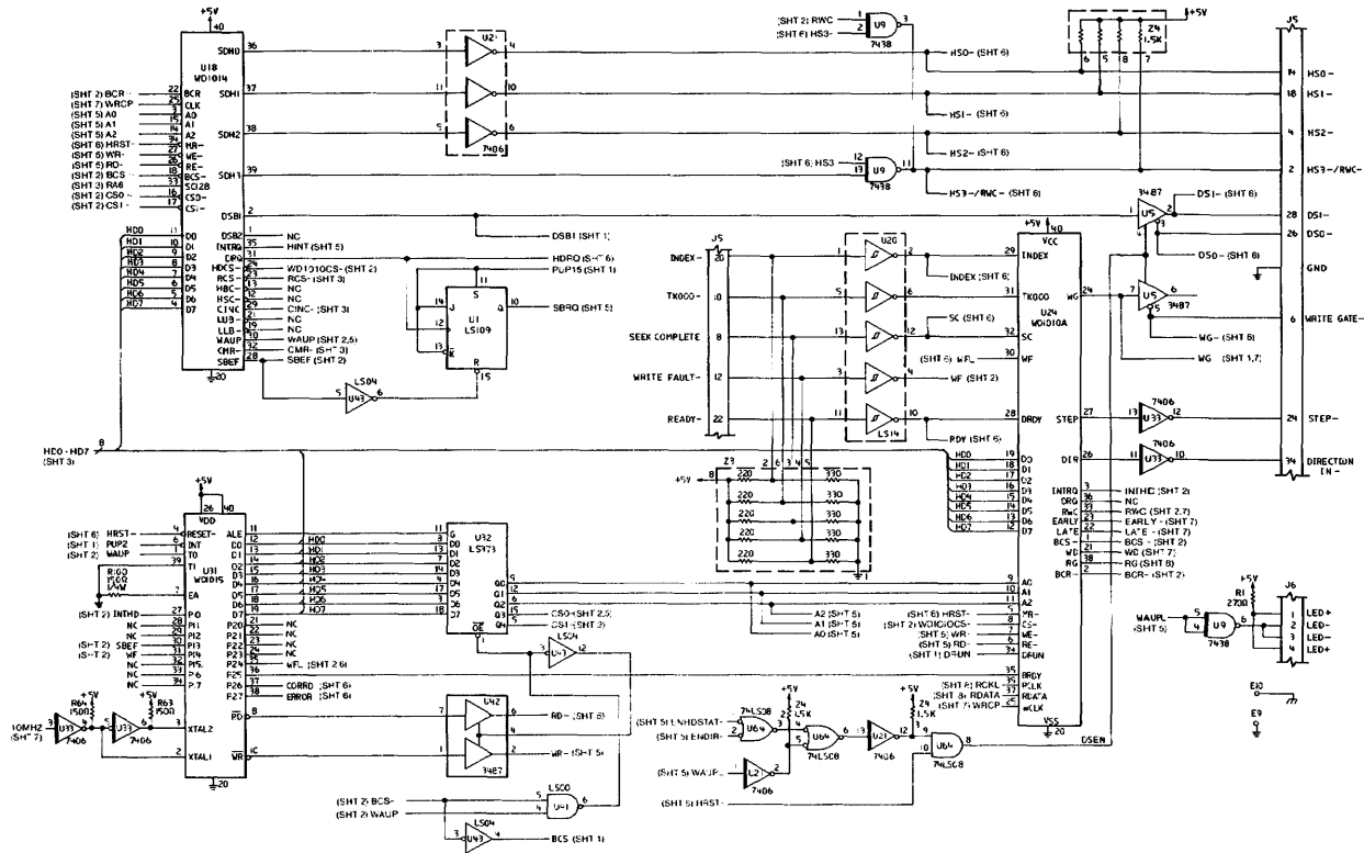
Fixed Disk and Diskette Drive Adapter - Level 1 (Sheet 2 of 9)
