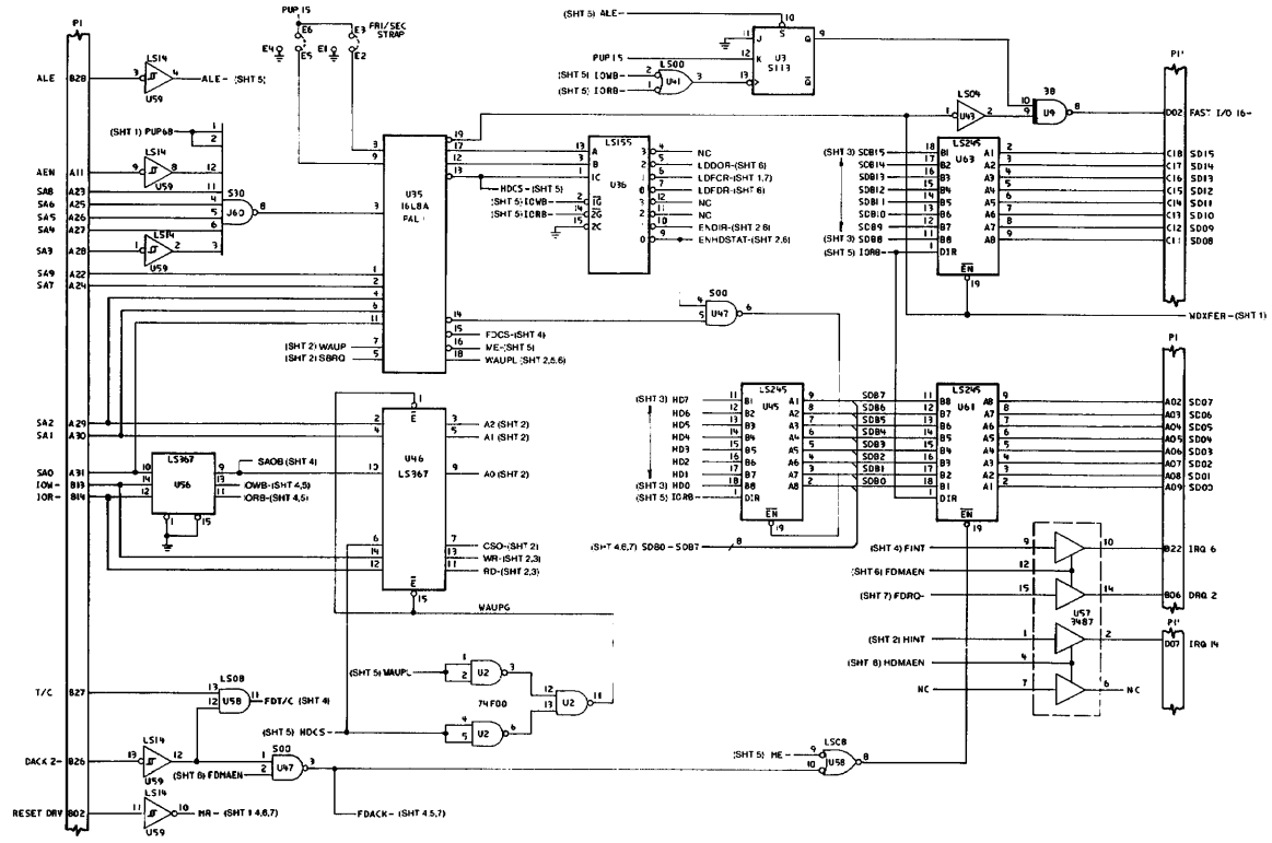
Fixed Disk and Diskette Drive Adapter - Level 1 (Sheet 5 of 9)
