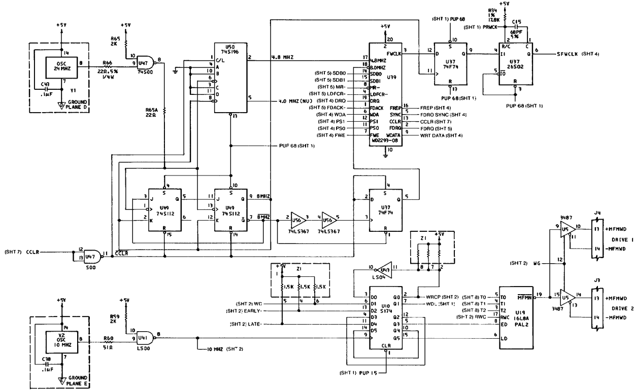
Fixed Disk and Diskette Drive Adapter - Level 1 (Sheet 7 of 9)
