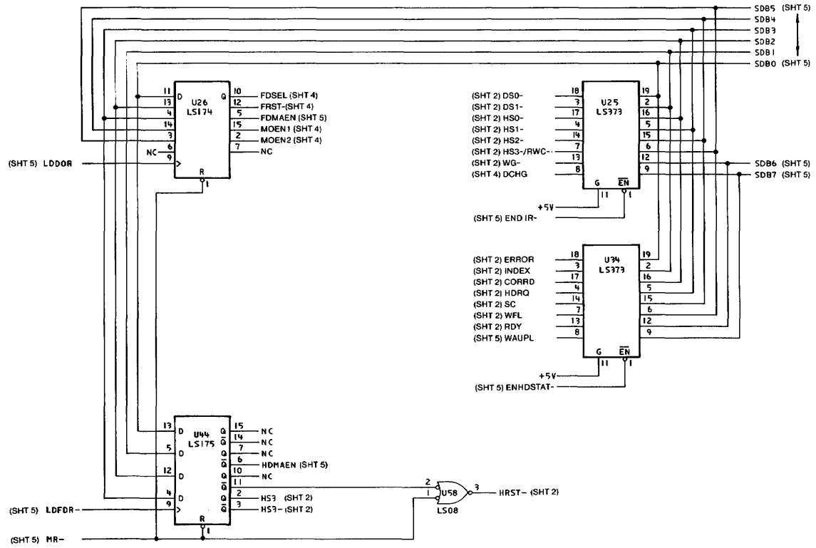
Fixed Disk and Diskette Drive Adapter - Level 1 (Sheet 6 of 9)
