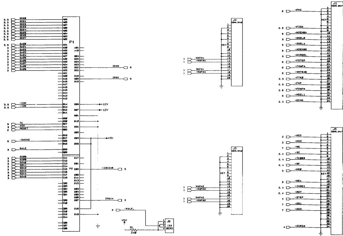
Fixed Disk and Diskette Drive Adapter—Level 2 (Sheet 1 of 7)
