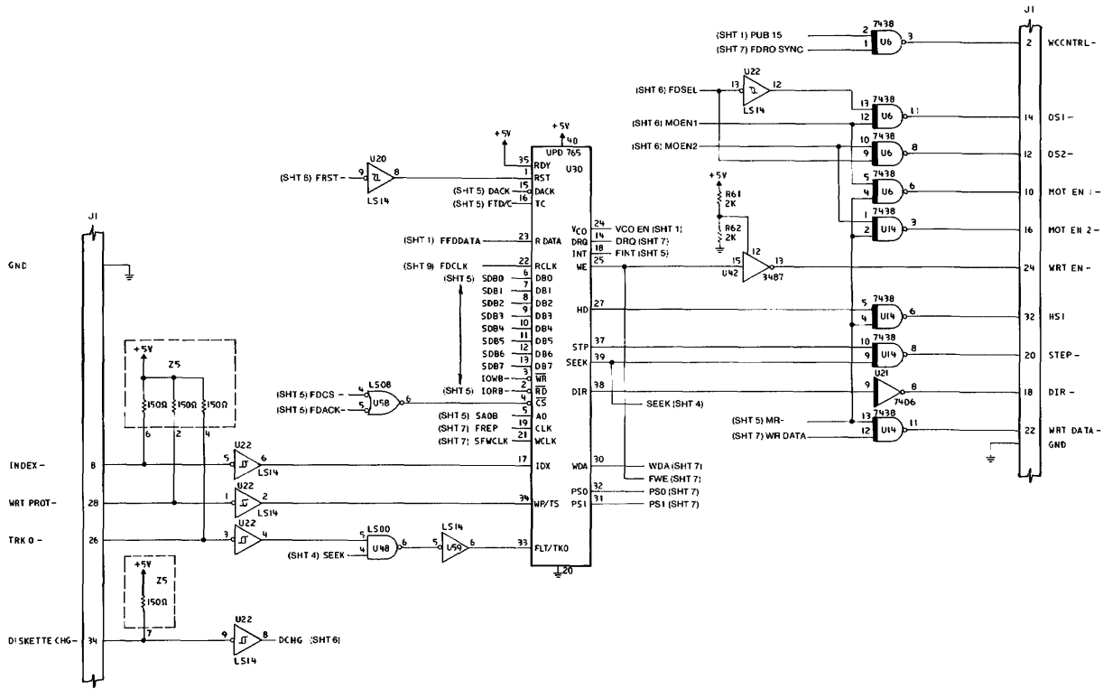
Fixed Disk and Diskette Drive Adapter - Level 1 (Sheet 4 of 9)
