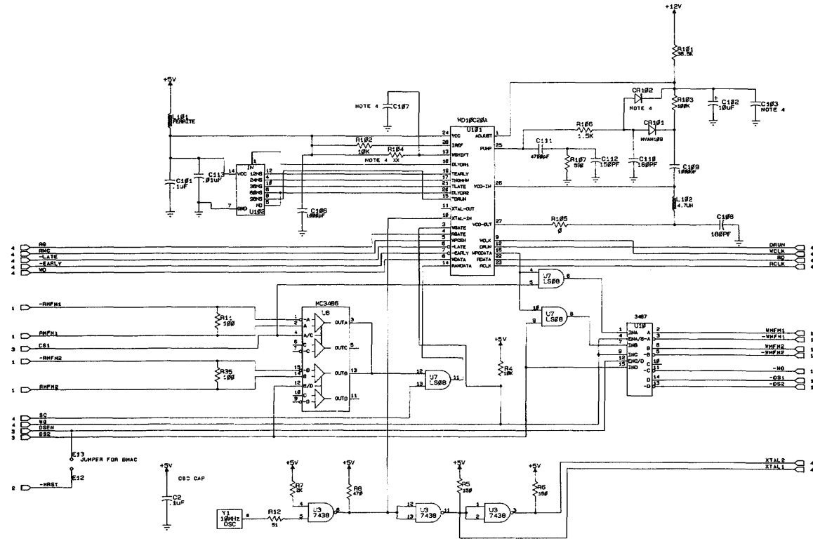
Fixed Disk and Diskette Drive Adapter—Level 2 (Sheet 7 of 7)
