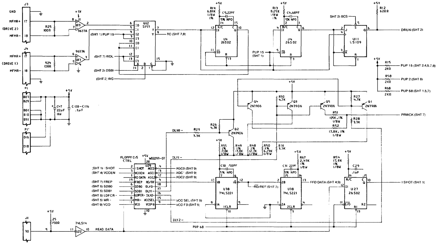
Fixed Disk and Diskette Drive Adapter - Level 1 (Sheet 1 of 9)
