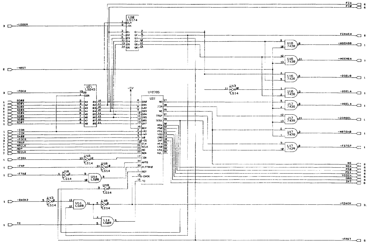
Fixed Disk and Diskette Drive Adapter-Level 2 (Sheet 5 of 7)
