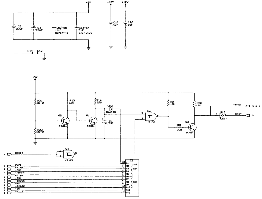
Fixed Disk and Diskette Drive Adapter—Level 2 (Sheet 2 of 7)
