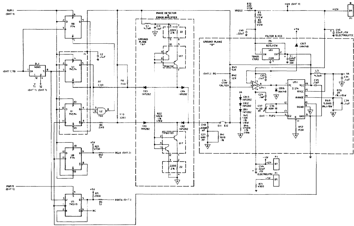
Fixed Disk and Diskette Drive Adapter - Level 1 (Sheet 8 of 9)
